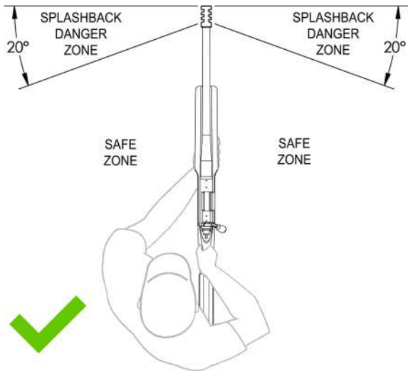
Figure 1a. Flat baffles feature a zero-degree impingement angle providing the largest safe zone.
