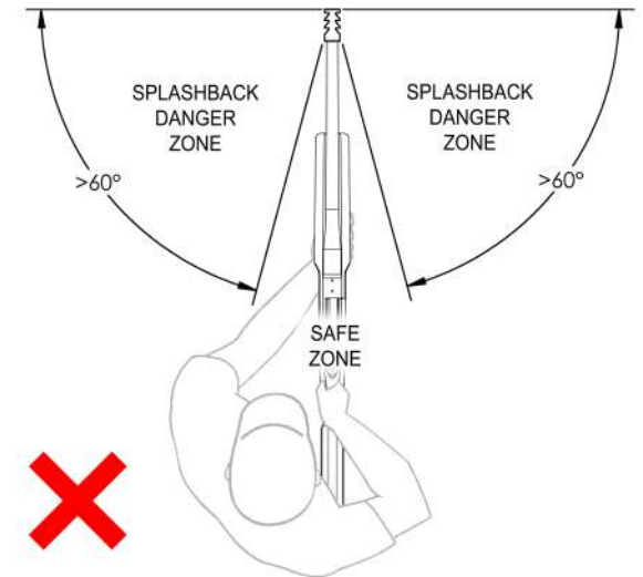
Figure 1c. Baffle angles greater than 40 degrees can cause splashback to directly strike the shooter causing serious injury. Muzzle brakes with baffle angles greater than 40-Deg should only be used if equipped with a rear mounted blast shield large enough to provide a minimum safe zone of 60-Deg.
